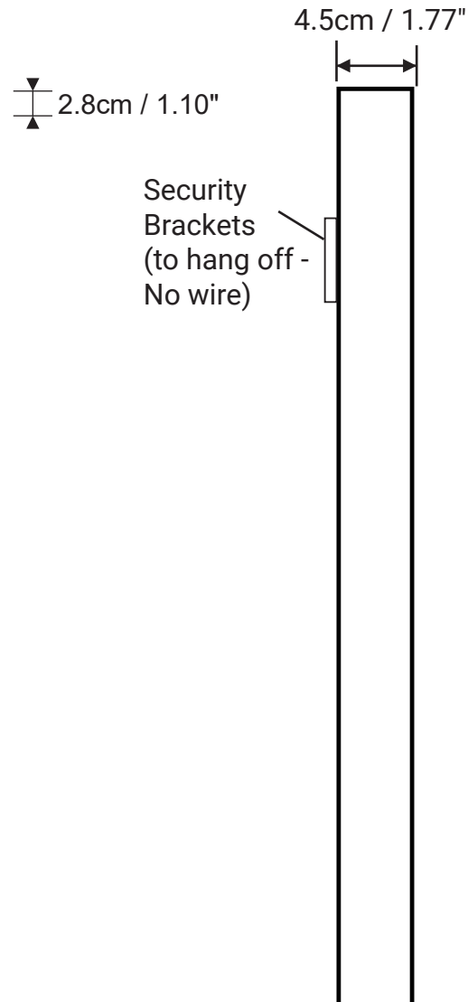
Side View
